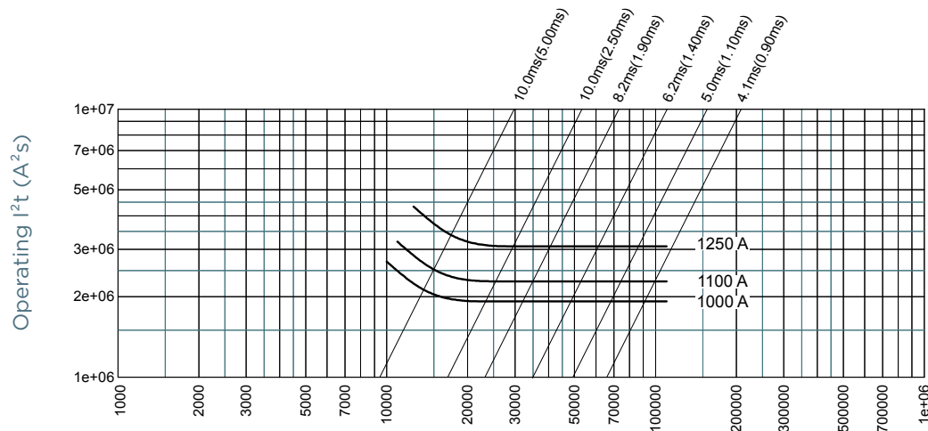
Size 73 aR 950V 50Hz RMS symmetrical prospective current (Ip)(A)
